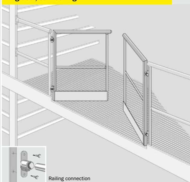
Railing connection
