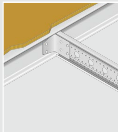
Platform supports made of a combination of hot-rolled profiles and system profiles
